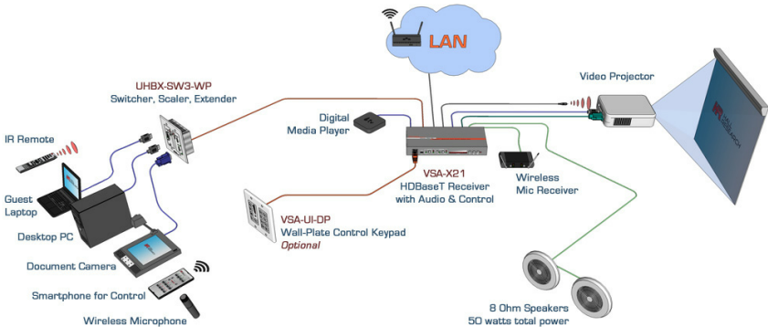
Figure 1 – Block Diagram
