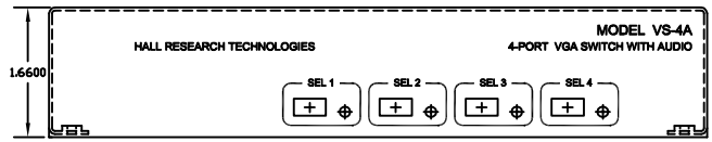
FRONT PANEL VIEW
